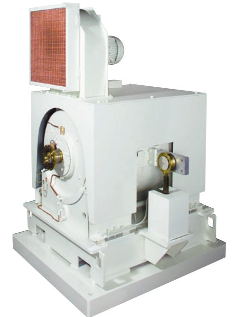
FREC Dynamometer, air-cooled type
