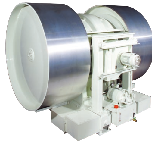
Overhung Type Chassis Dynamometer (Air-Cooled Type)
