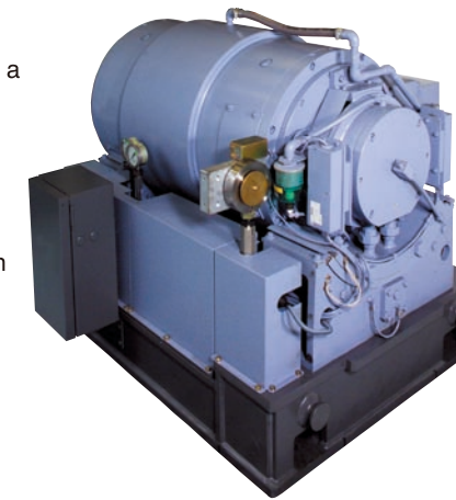
FREC Dynamometer, Liquid-cooled type
