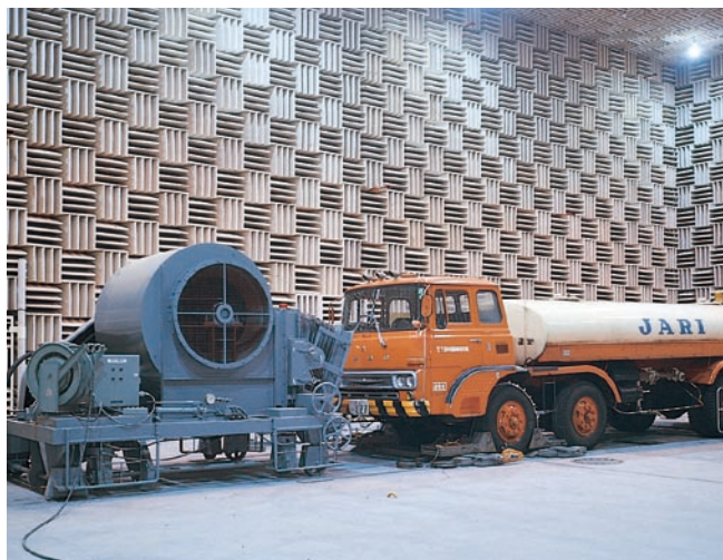
Chassis Dynamometer in a Large-Scale Anechoic Room
