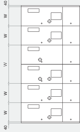
Fig.3 Switchgear Alignment
