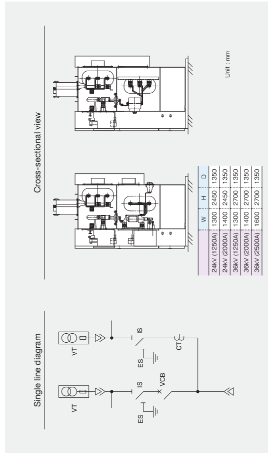
Bus section panel with CT & Bus VT
