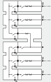
Fig.1 Single line diagram
