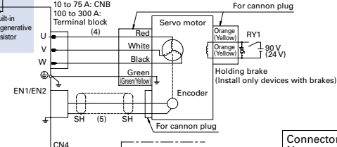
Servo amplifier
