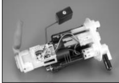
Fuel Supply Parts
