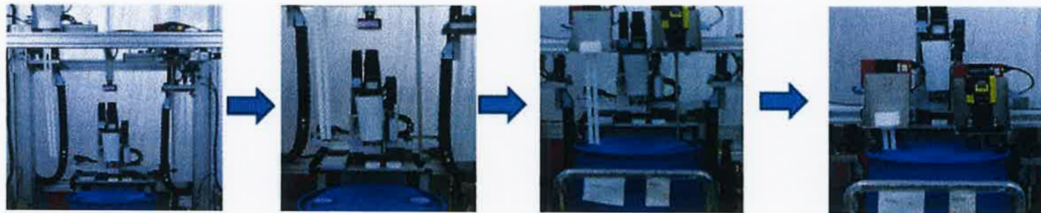
Wholly automated tube insertion (chemical supply tube, agitator shaft)
